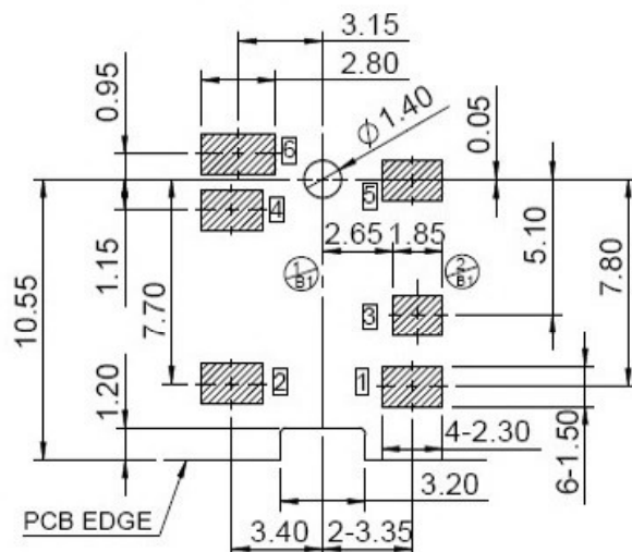
RECOMMENDED PCB LAYOUT(TOP VIEW) (GENERAL TOLERANCE ±0.05)
