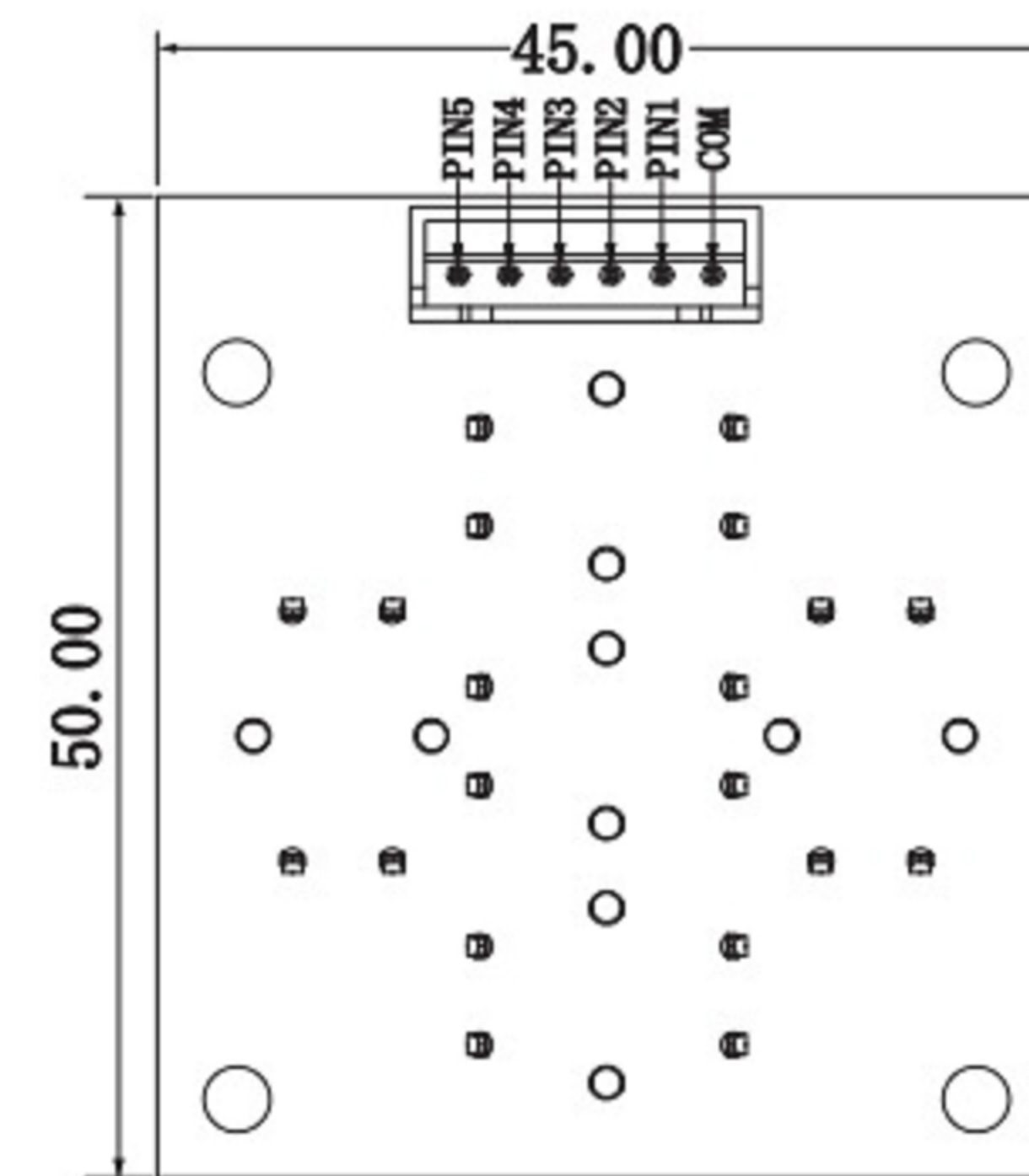
PCB LAYOUT
