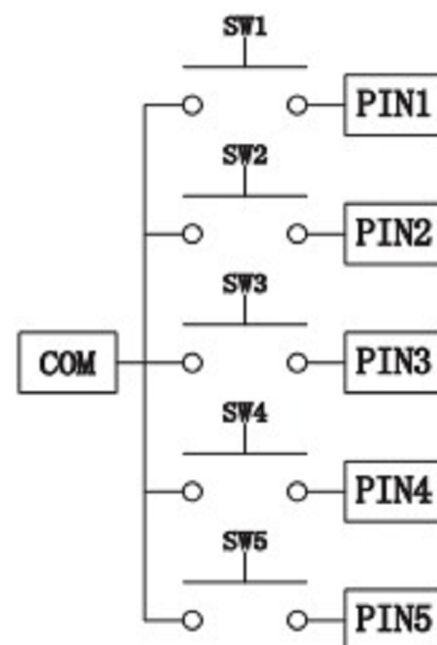
SCHEMATIC
