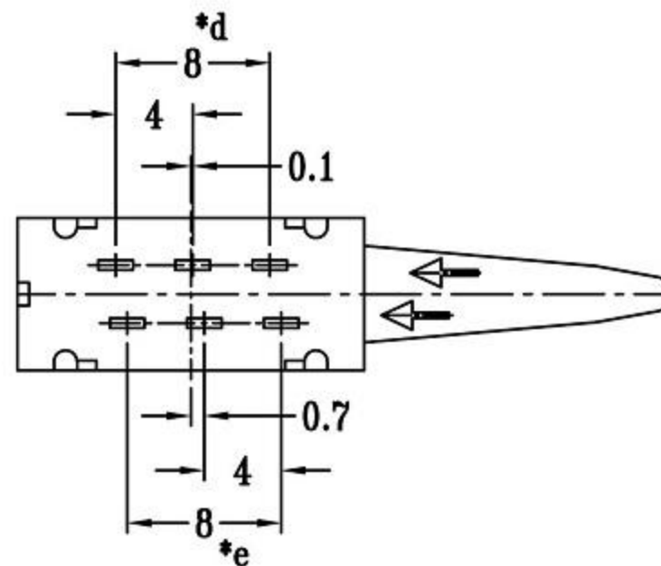
VIEW K
