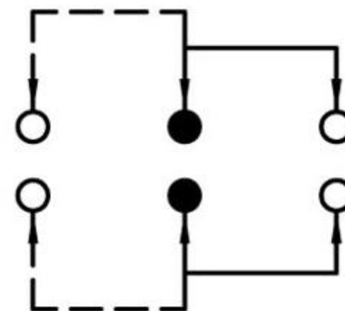
SCHEMATIC (NON-SHORTING)
