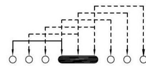
SCHEMATIC (NON-SHORTING)
