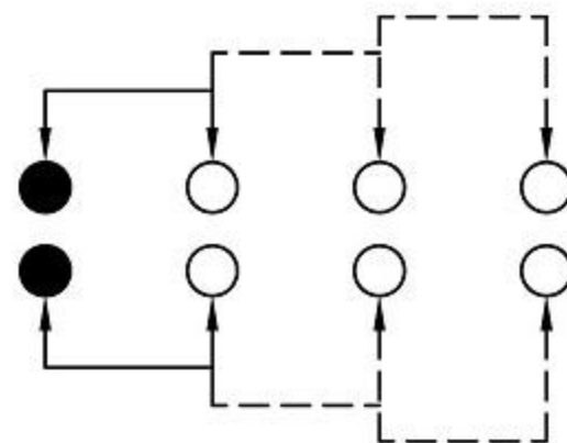
SCHEMATIC (NON-SHORTING)
