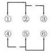
SCHEMATIC (NON-SHORTING)
