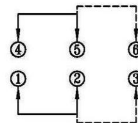
SCHEMATIC (NON-SHORTING)
