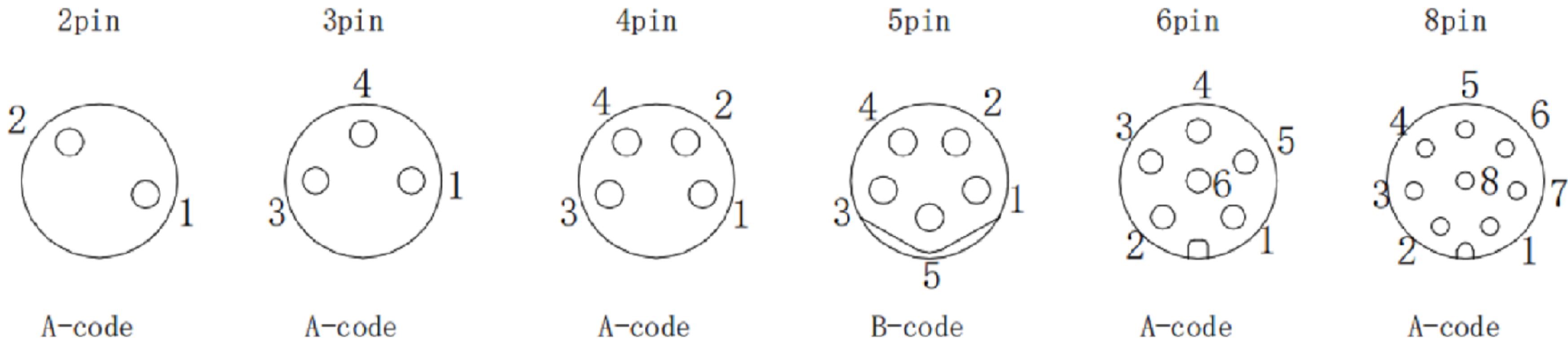
Pin assignment front view/针位分布前视图
