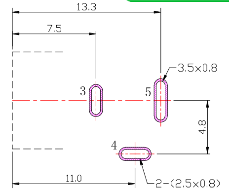
P.C.B LAYOUT MOUNTING PATTERN (TOP VIEW)
