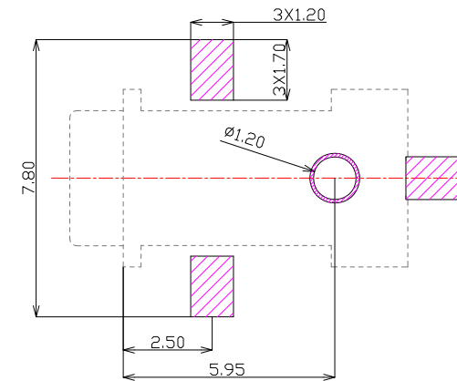
LAYOUT PCB BOTTOM VIEW
