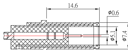
RECOMMENDED PLUG
