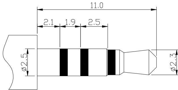
Ø2.50mm 4 POLE PLUG
