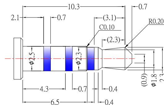
ø2.50mm 4 POLE PLUG DETAIL DRAWING
