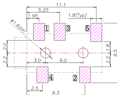
RECOMMENDED P. C. B. LAYOUT (COPPER-SIDED VIEW)
